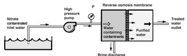
Figure 2. A schematic of the reverse osmosis process.
